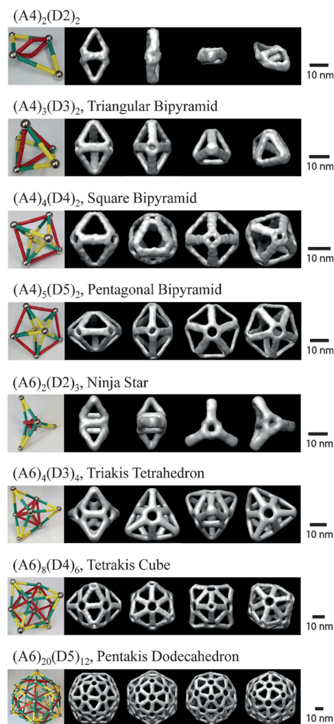
Figure 4. Reconstructed 3D structural models of the DNA complexes that resulted from directed self-assembly. For each structure, four views at different orientations are shown. The corresponding designs are shown on the left. See Figures S4–S17 for details.
